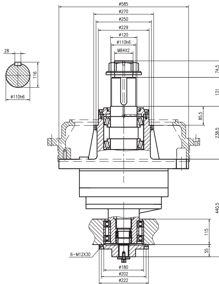
LSJ28 拉丝机专用减速机技术数据 Wire Drawing Machine Gearbox Technical Data
