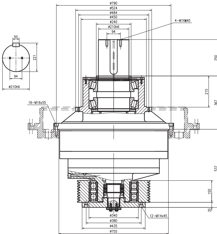
LSJ108 拉丝机专用减速机技术数据 Wire Drawing Machine Gearbox Technical Data
