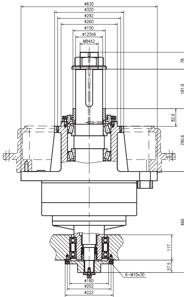
LSJ48 拉丝机专用减速机技术数据 Wire Drawing Machine Gearbox Technical Data
