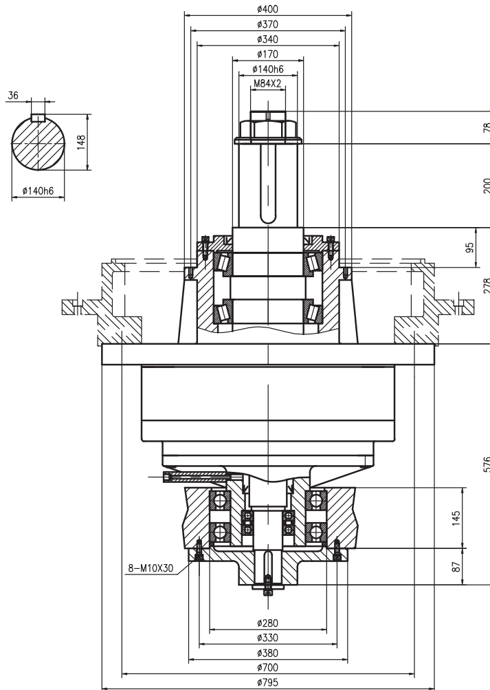
LSJ68 拉丝机专用减速机技术数据 Wire Drawing Machine Gearbox Technical Data
